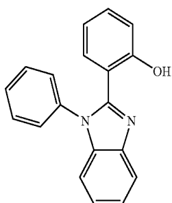
Structure Formula (19)
