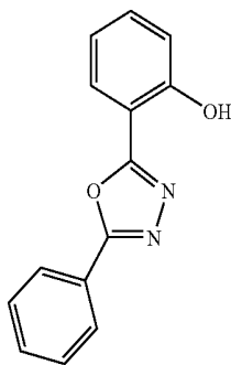
Structure Formula (20)
